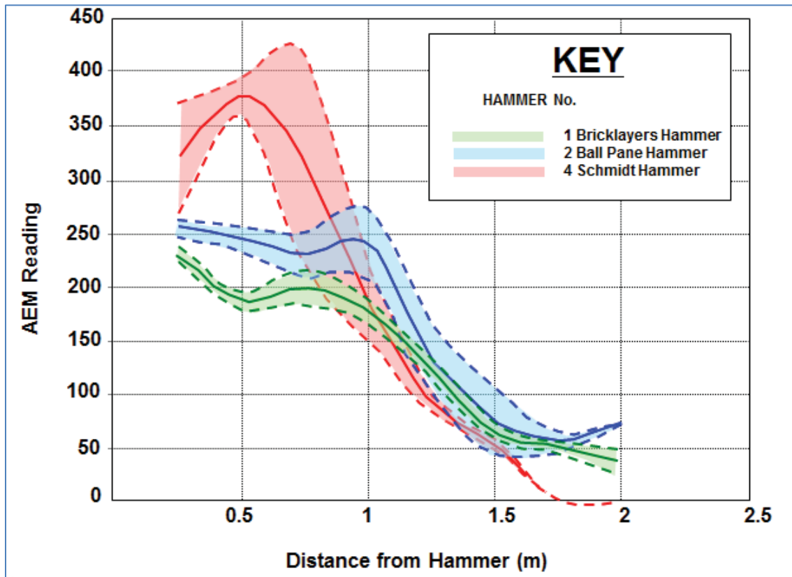
Figure 165: Effect of hammer type on AEM readings (Bigby, 2007)
