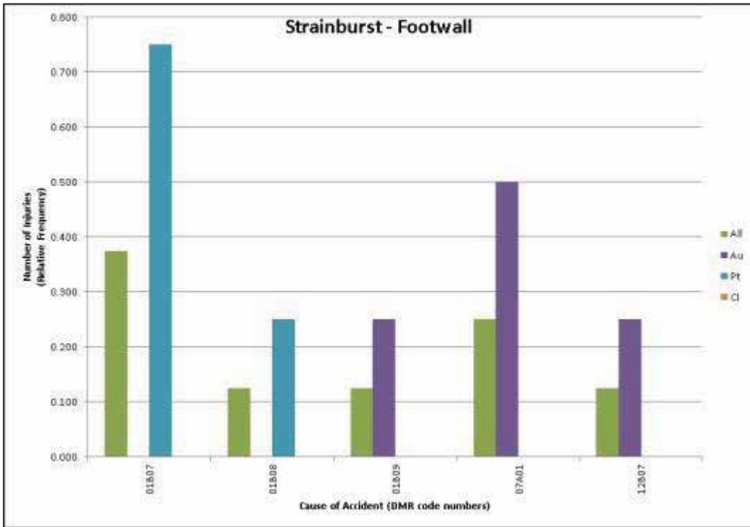
Figure 113: Probable Causes of Strainburst-Footwall Accidents
