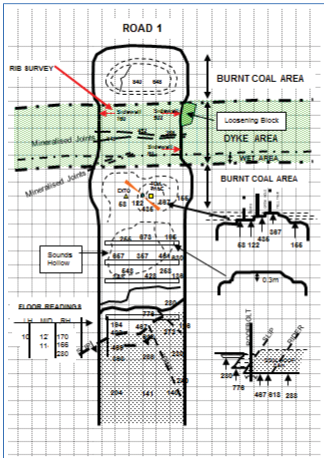
Figure 166: Results of using AEM near a dyke in a Colliery (Bigby, 2007)
