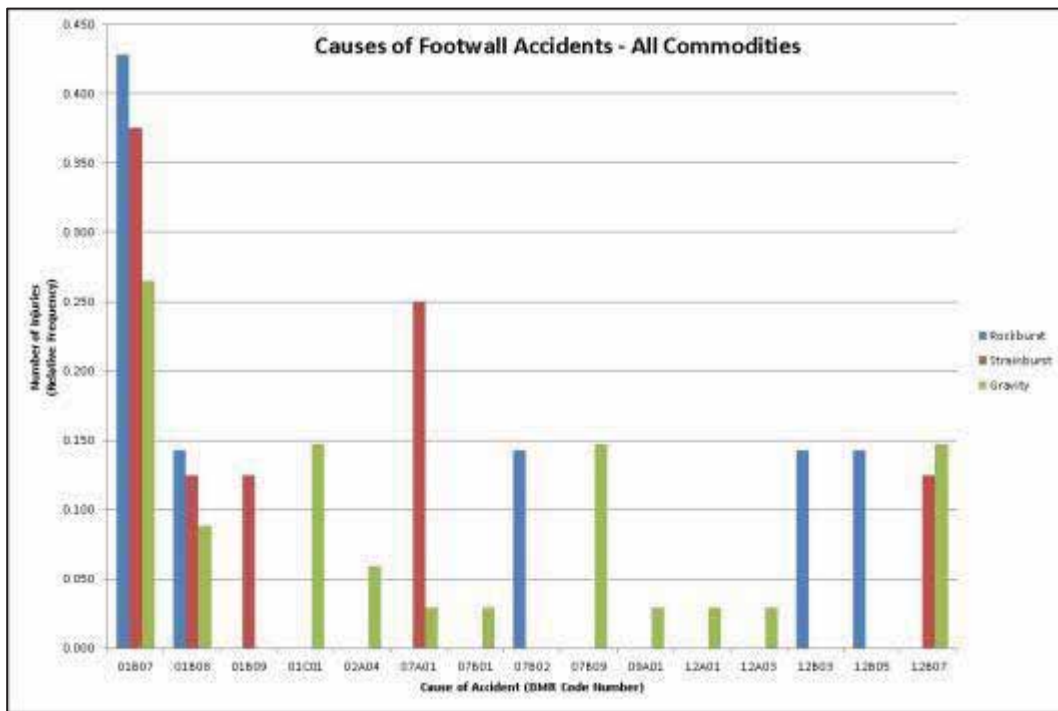
Figure 122: Probable Causes of Footwall Accidents - All Commodities
