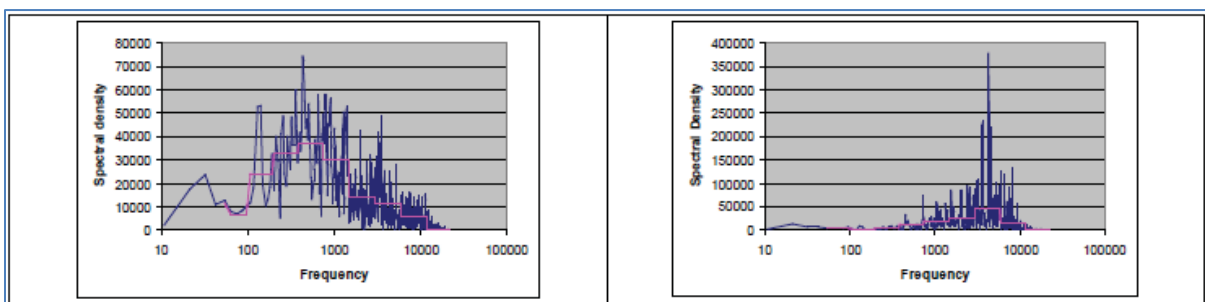
Figure 169: Spectral density of sounding responses (Vogt, et. al., 2010)
