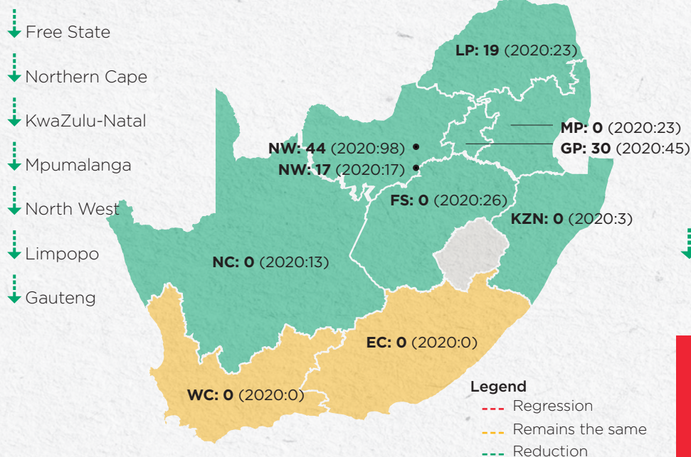
Injuries per region to date (15 February 2021)
