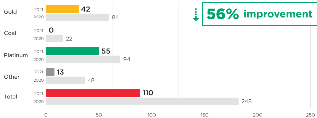
Injuries per commodity to date (15 February 2021)
