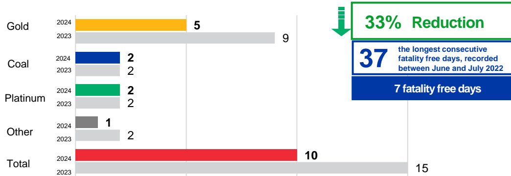
Fatalities per commodity to date (08 April 2024)
