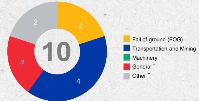
Fatalities by classification to date (08 April 2024)
