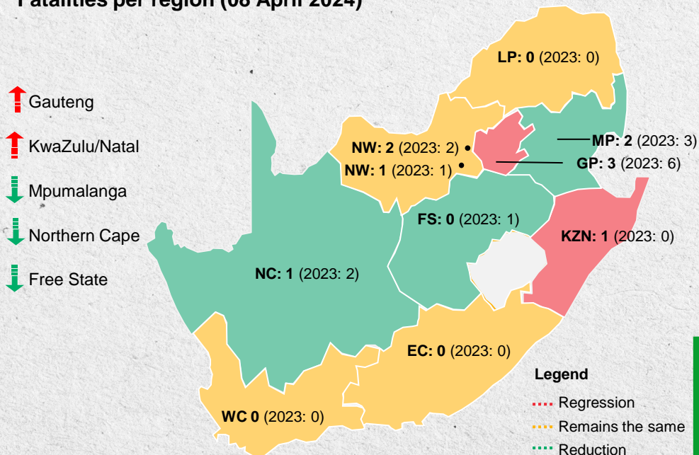
Fatalities per region (08 April 2024)
