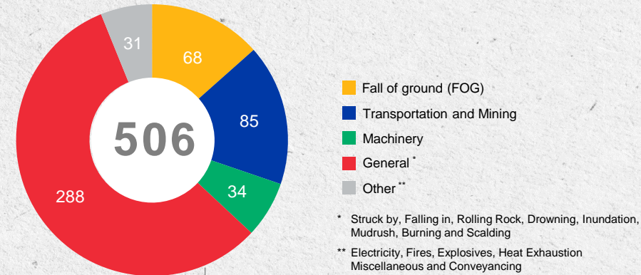
Injuries by classification to date (08 April 2024)
