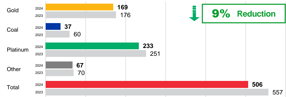
Injuries per commodity to date (08 April 2024)
